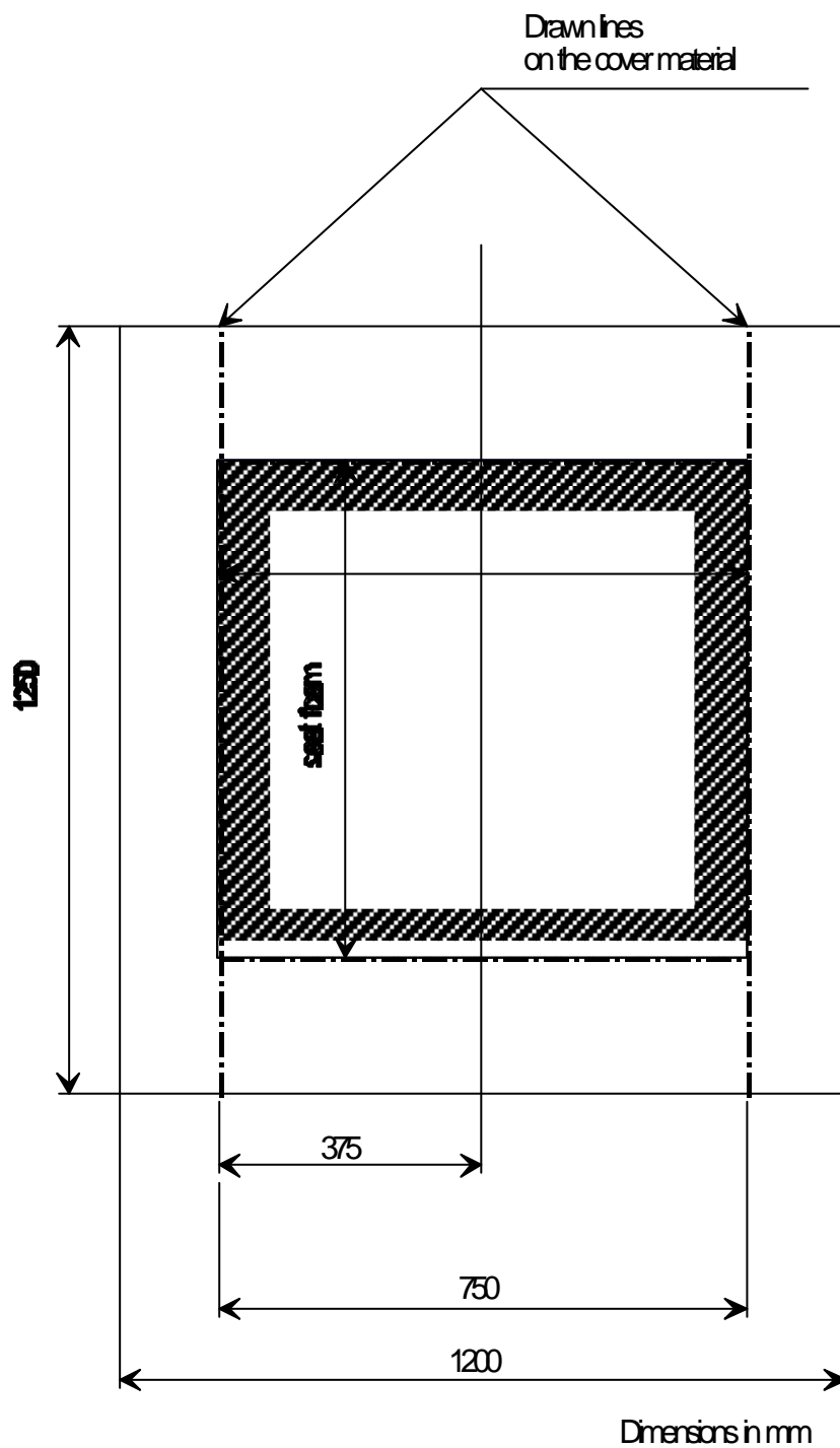
Figure 3 : Dimensions of the cover material
