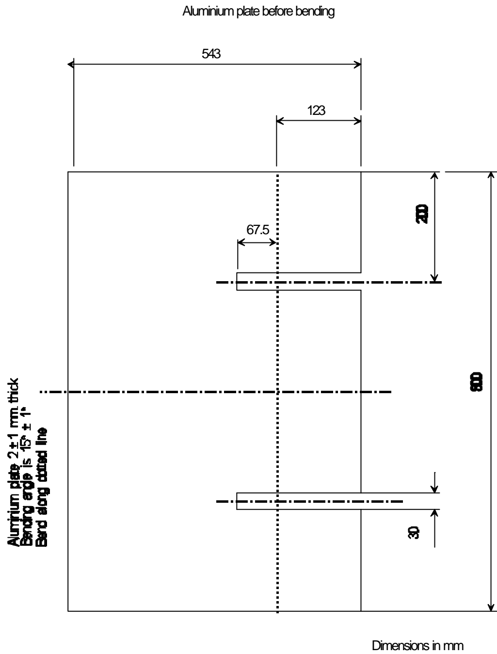
Figure 2 : Dimensions of the aluminium bottom-plate
