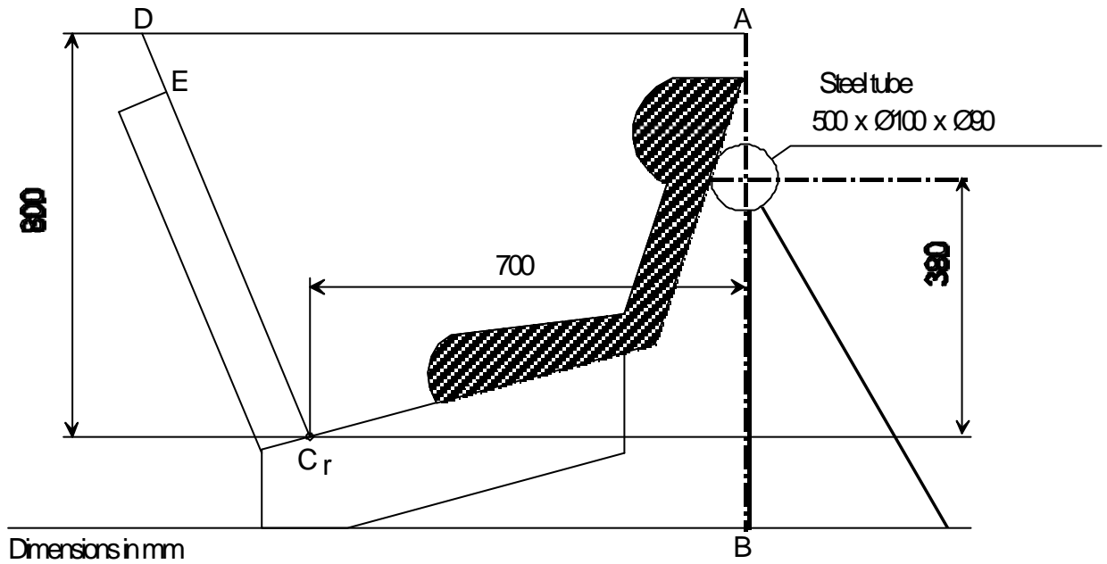
Figure 2 Arrangement for testing a rearward-facing device
